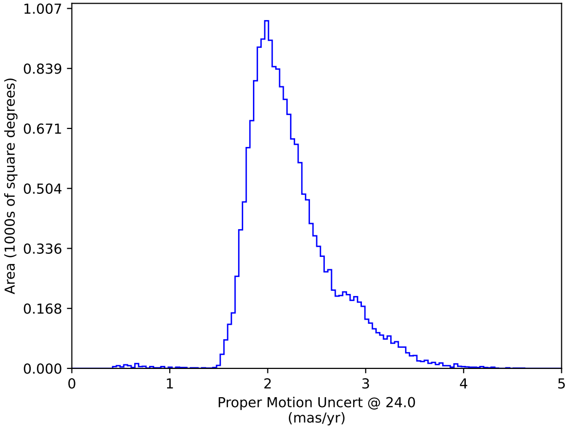
weather_cloudso35v3.4_10yrs WFD: Proper Motion Uncert @ 24.0
