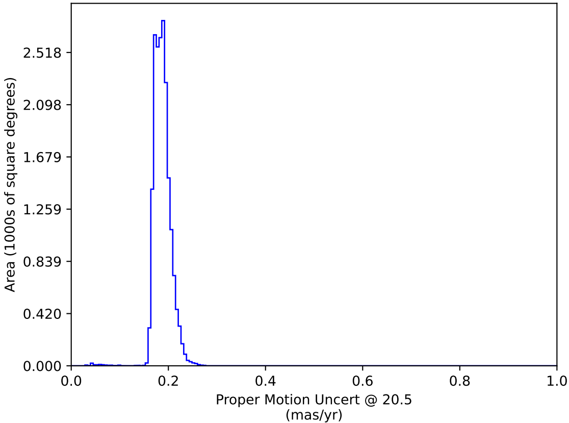
weather_cloudso35v3.4_10yrs WFD: Proper Motion Uncert @ 20.5
