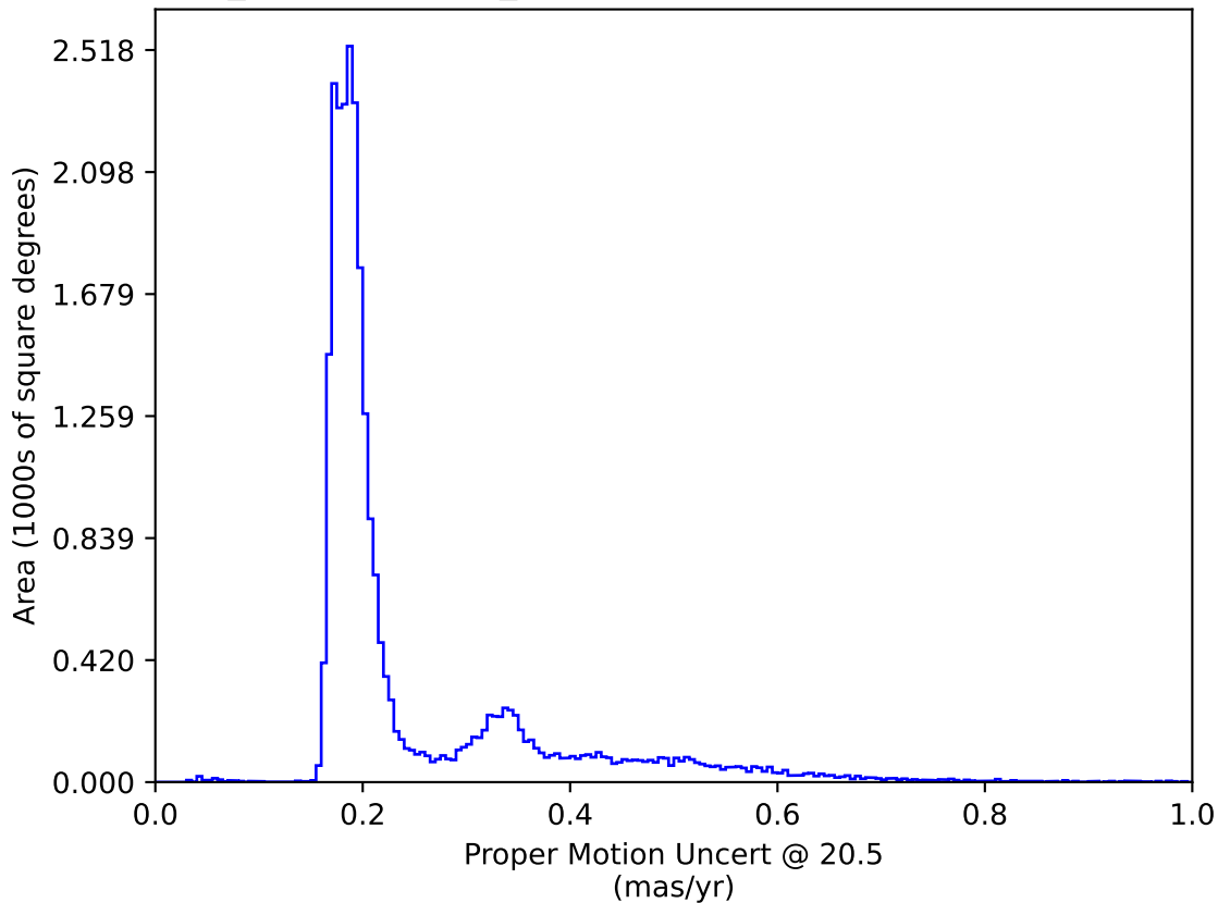
weather_cloudso35v3.4_10yrs All sky: Proper Motion Uncert @ 20.5
