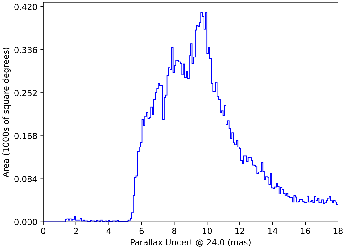
weather_cloudso35v3.4_10yrs All sky: Parallax Uncert @ 24.0
