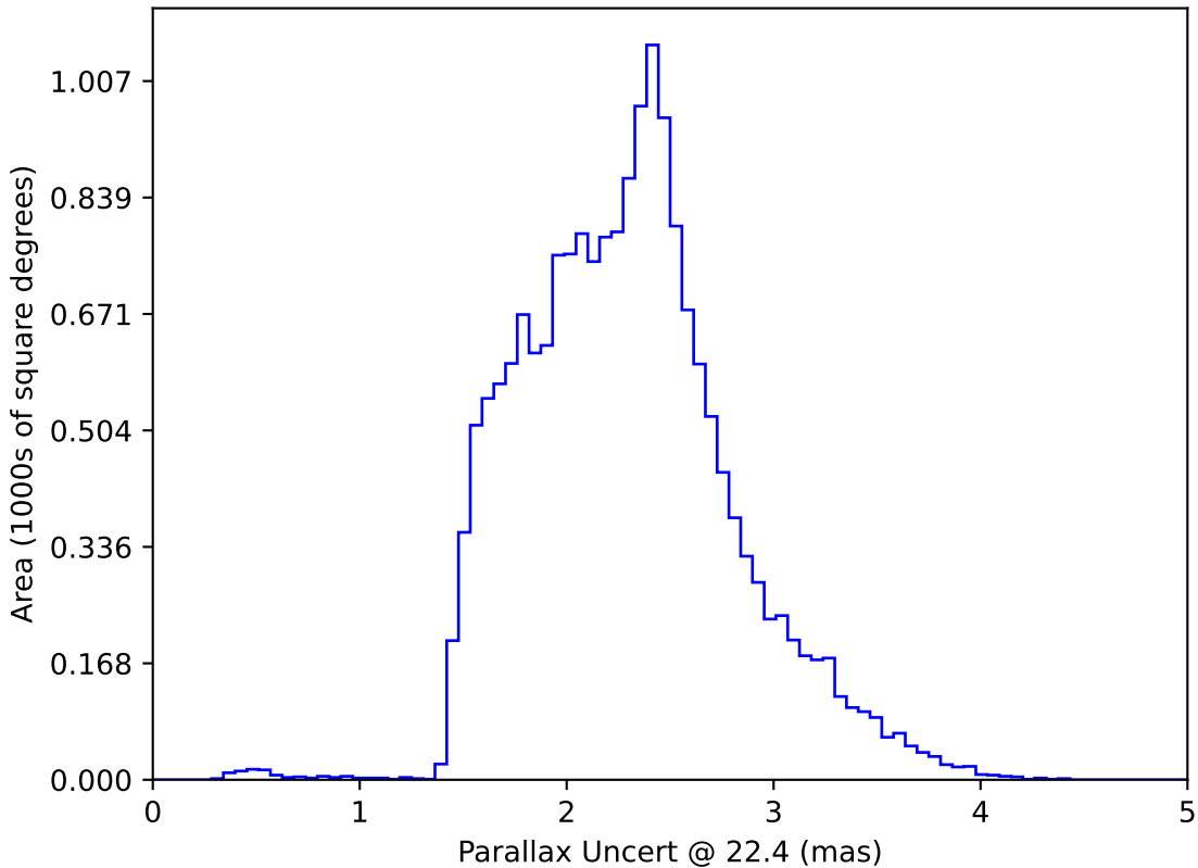
weather_cloudso35v3.4_10yrs WFD: Parallax Uncert @ 22.4
