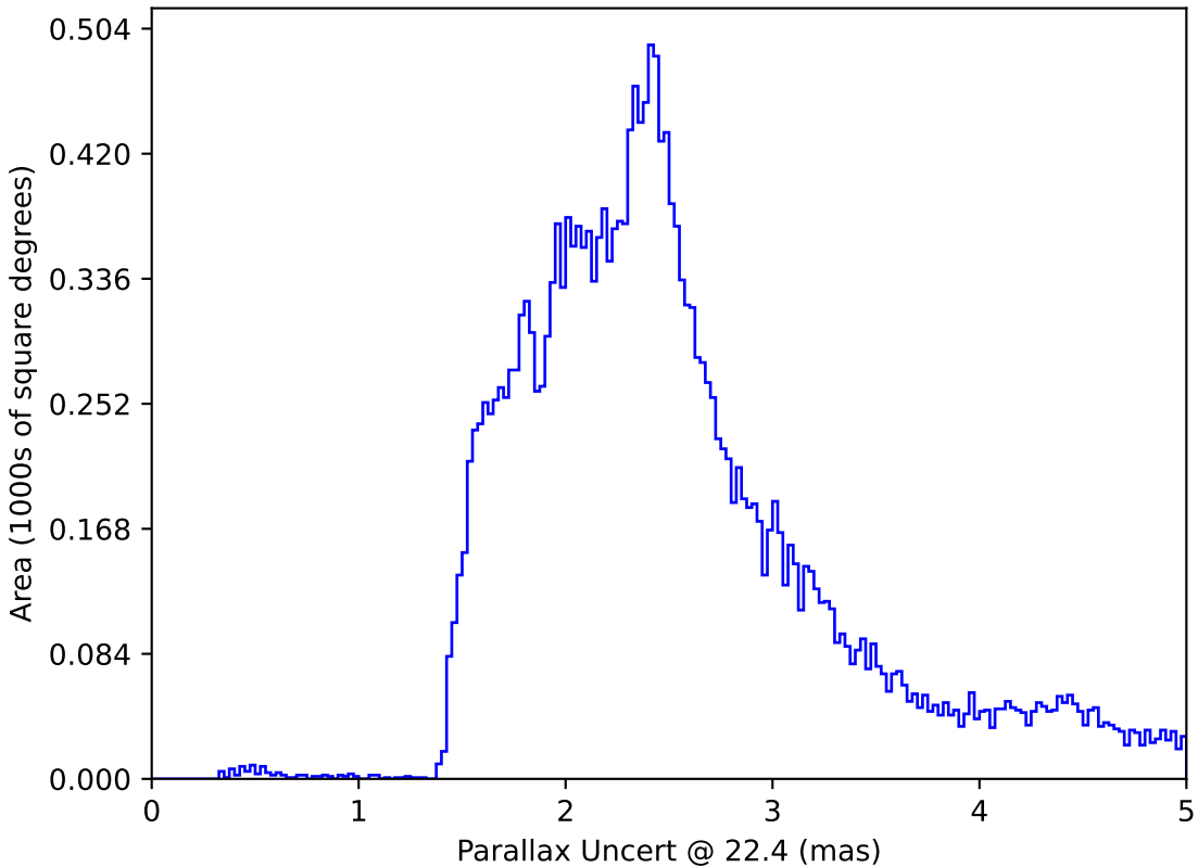
weather_cloudso35v3.4_10yrs All sky: Parallax Uncert @ 22.4
