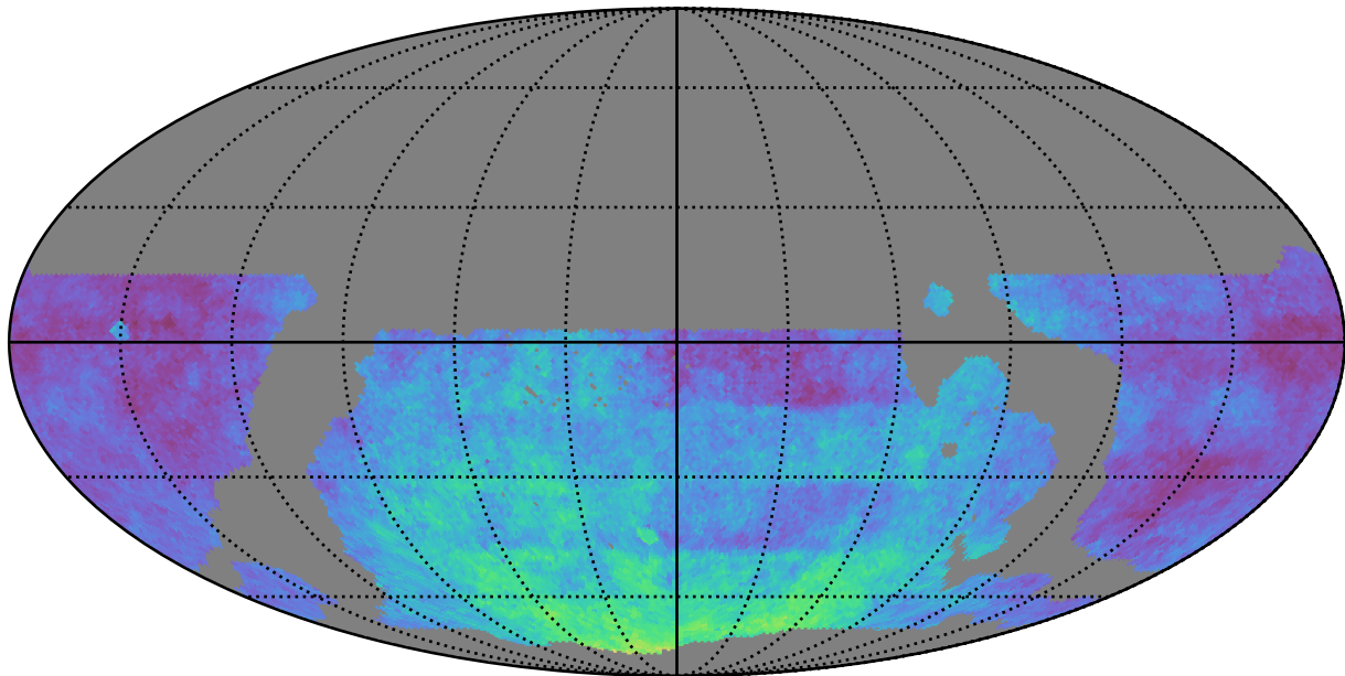
weather_cloudso35v3.4_10yrs WFD: Parallax Coverage @ 24.0
