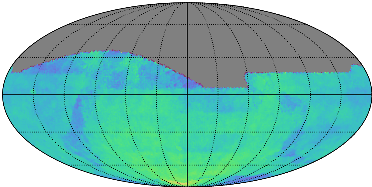
weather_cloudso35v3.4_10yrs All sky: Parallax Coverage @ 24.0
