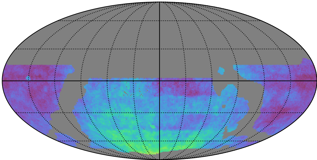
weather_cloudso35v3.4_10yrs WFD: Parallax Coverage @ 22.4
