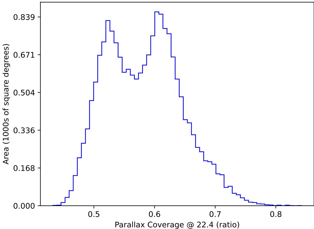
weather_cloudso35v3.4_10yrs WFD: Parallax Coverage @ 22.4
