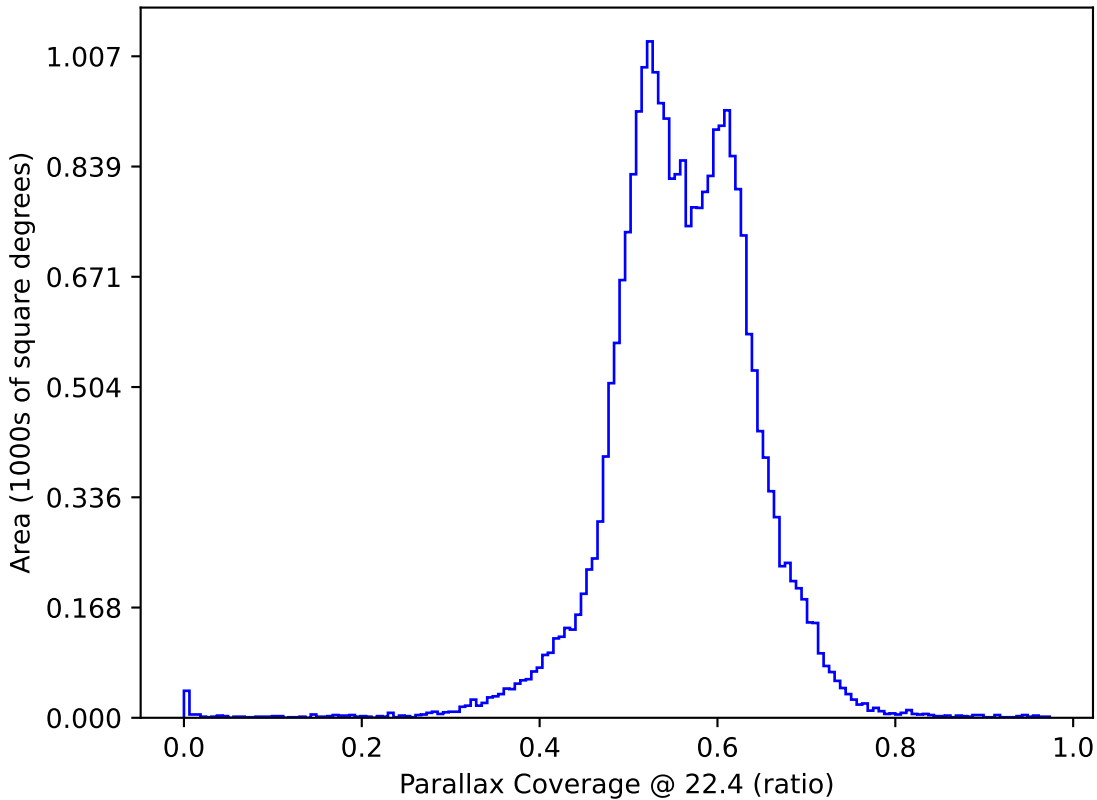
weather_cloudso35v3.4_10yrs All sky: Parallax Coverage @ 22.4
