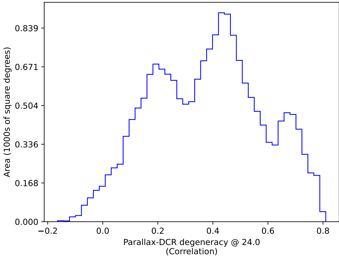
weather_cloudso35v3.4_10yrs WFD: Parallax-DCR degeneracy @ 24.0
