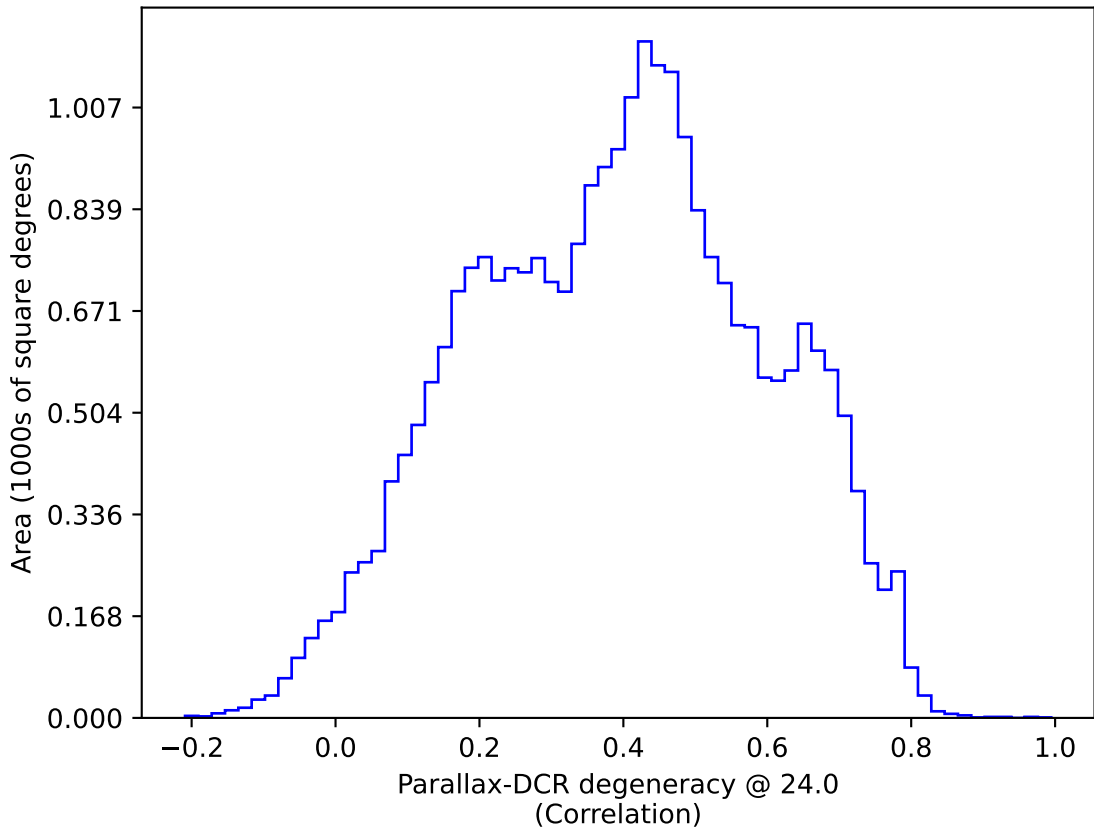
weather_cloudso35v3.4_10yrs All sky: Parallax-DCR degeneracy @ 24.0
