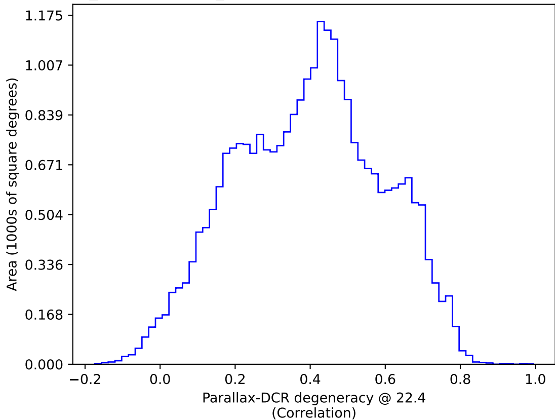
weather_cloudso35v3.4_10yrs All sky: Parallax-DCR degeneracy @ 22.4
