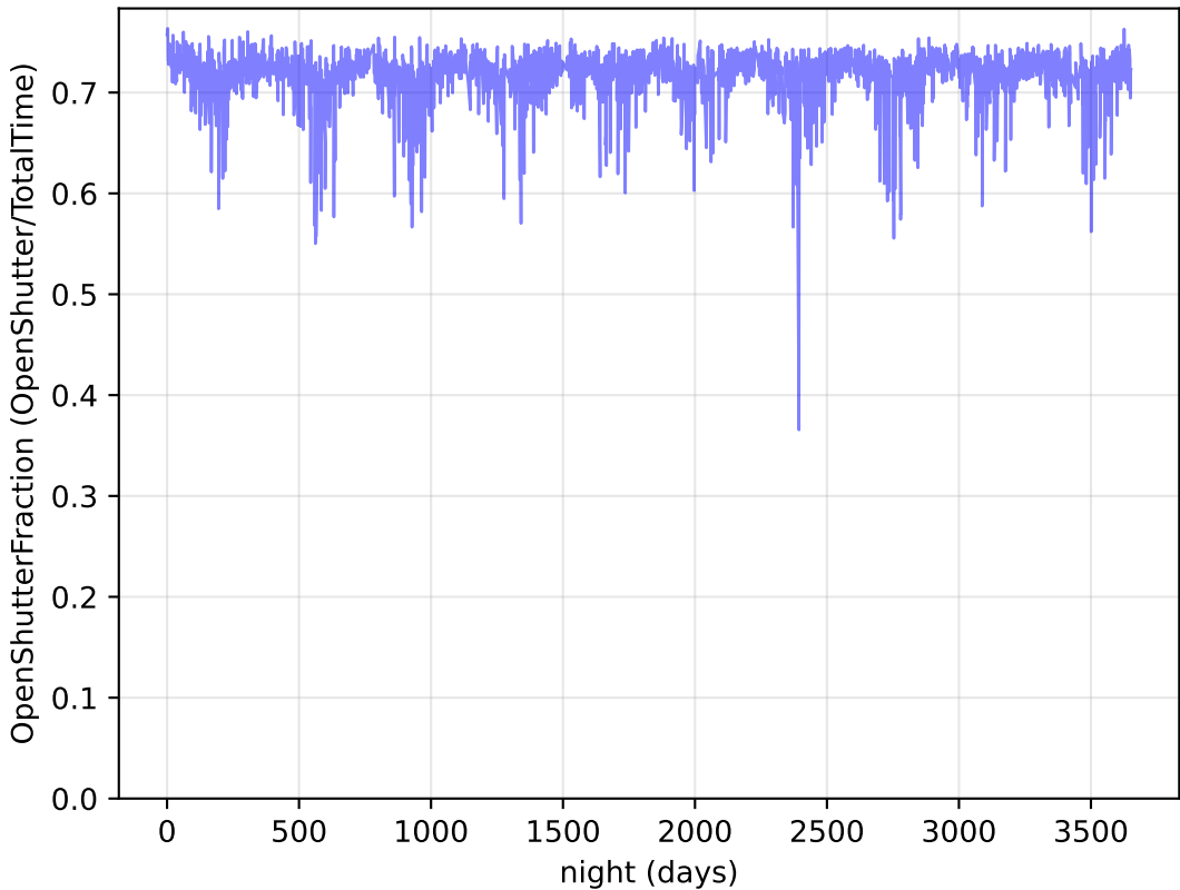
weather_cloudso35v3.4_10yrs Per night: OpenShutterFraction
