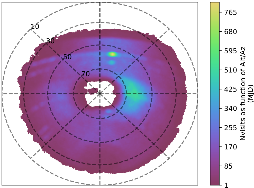
weather_cloudso35v3.4_10yrs u band: Nvisits as function of Alt/Az
