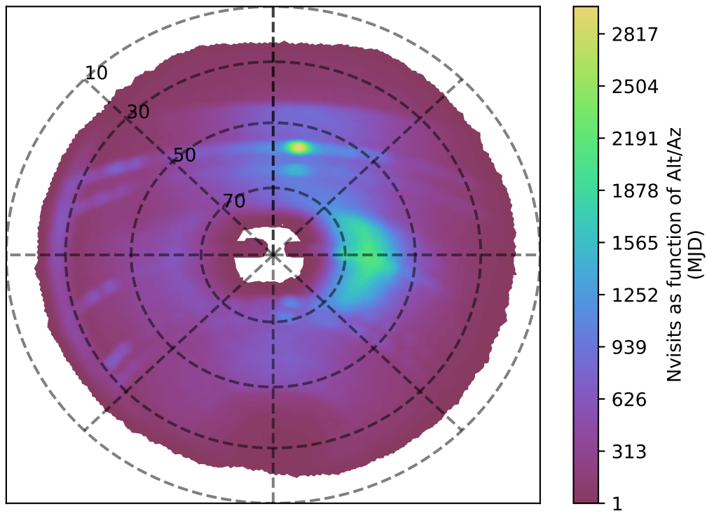
weather_cloudso35v3.4_10yrs r band: Nvisits as function of Alt/Az
