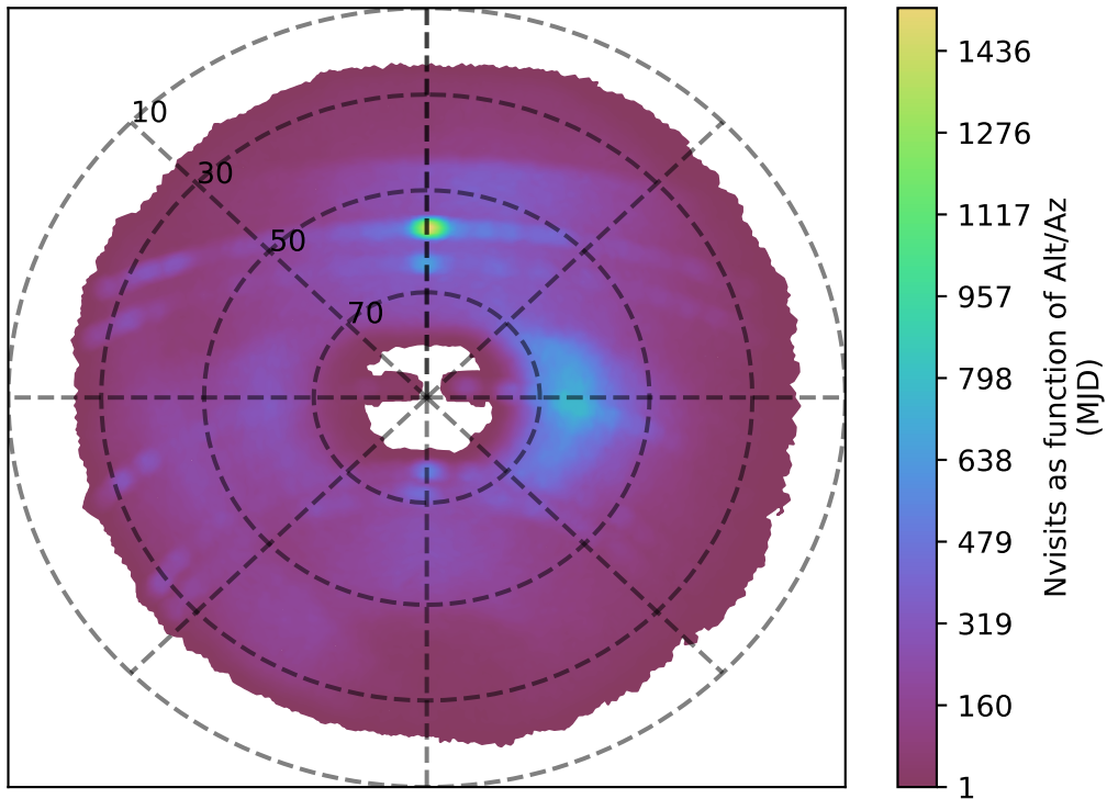
weather_cloudso35v3.4_10yrs g band: Nvisits as function of Alt/Az
