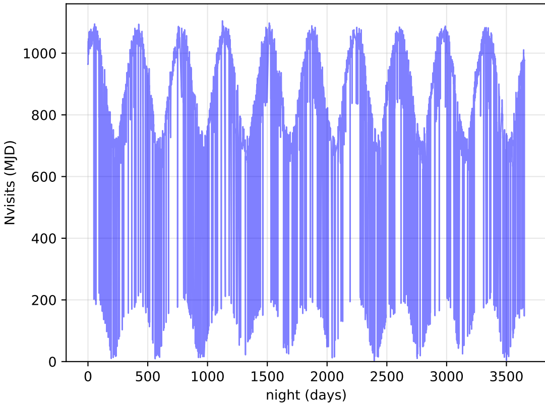
weather_cloudso35v3.4_10yrs All visits: Nvisits
