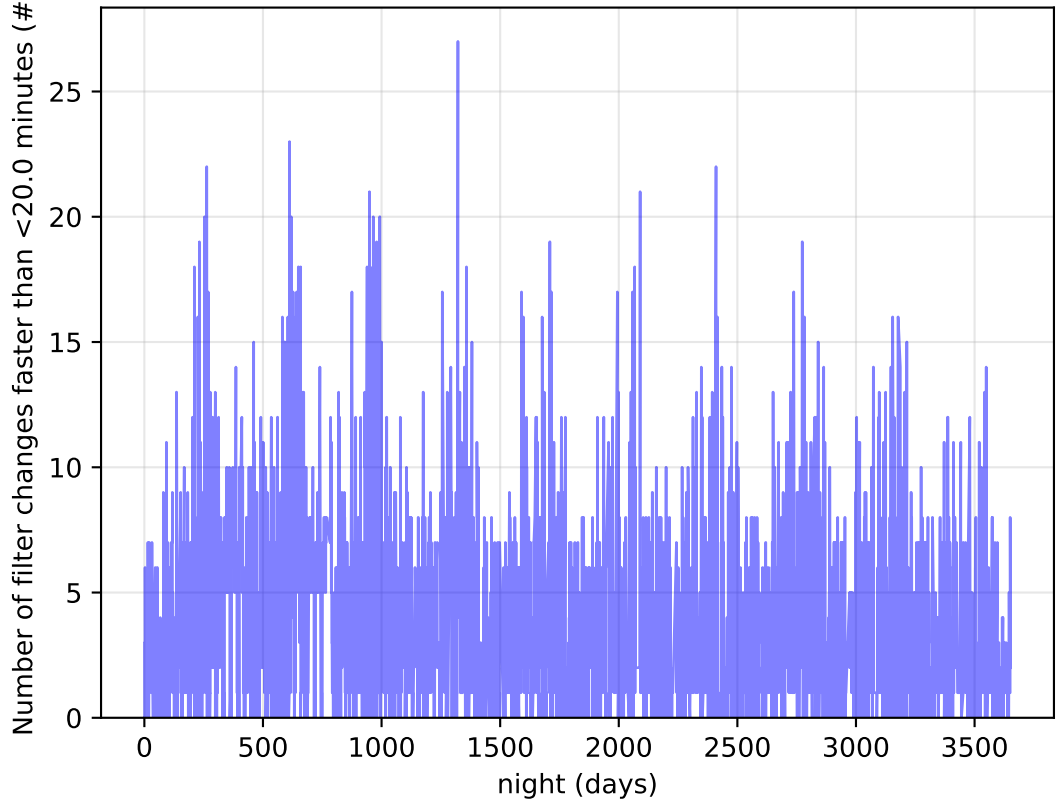
weather_cloudso35v3.4_10yrs Per Night: Number of filter changes faster than <20.0 minutes
