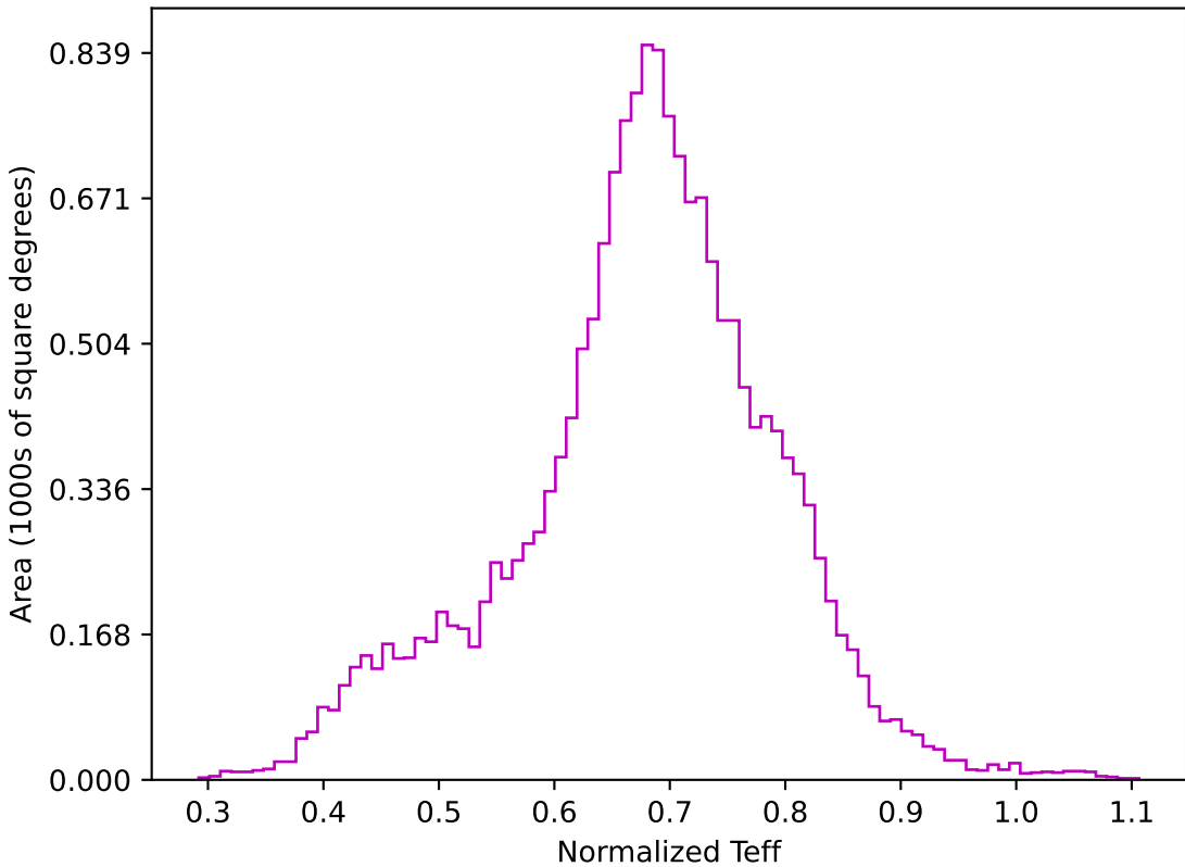
weather_cloudso35v3.4_10yrs WFD z band: Normalized Teff
