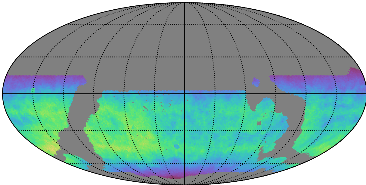
weather_cloudso35v3.4_10yrs WFD y band: Normalized Teff
