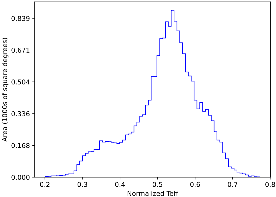
weather_cloudso35v3.4_10yrs WFD y band: Normalized Teff
