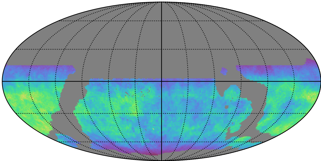
weather_cloudso35v3.4_10yrs WFD u band: Normalized Teff
