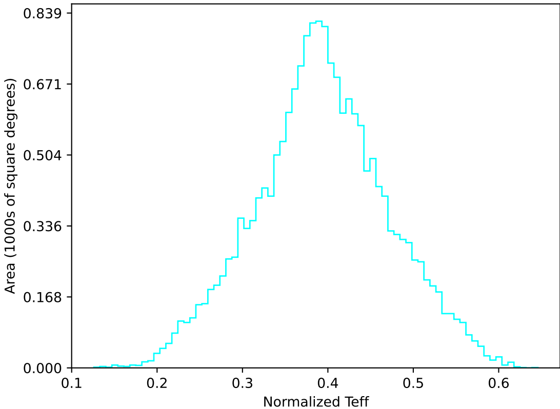
weather_cloudso35v3.4_10yrs WFD u band: Normalized Teff
