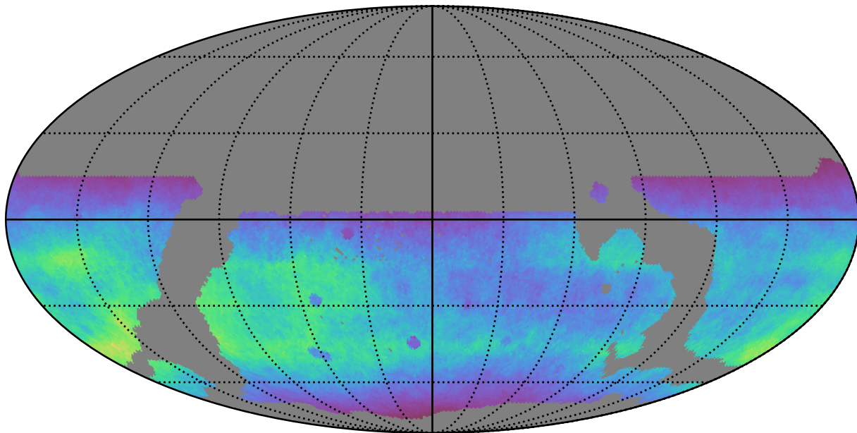
weather_cloudso35v3.4_10yrs WFD r band: Normalized Teff
