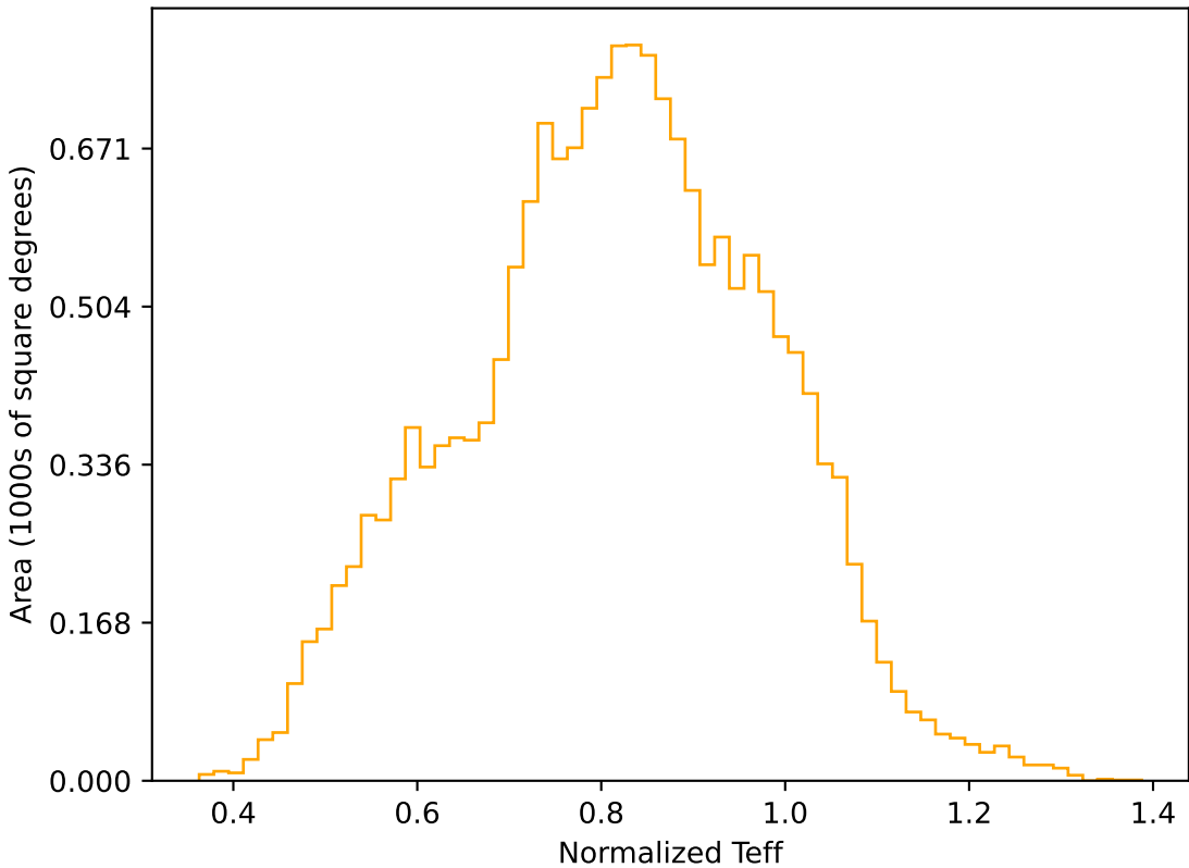
weather_cloudso35v3.4_10yrs WFD r band: Normalized Teff
