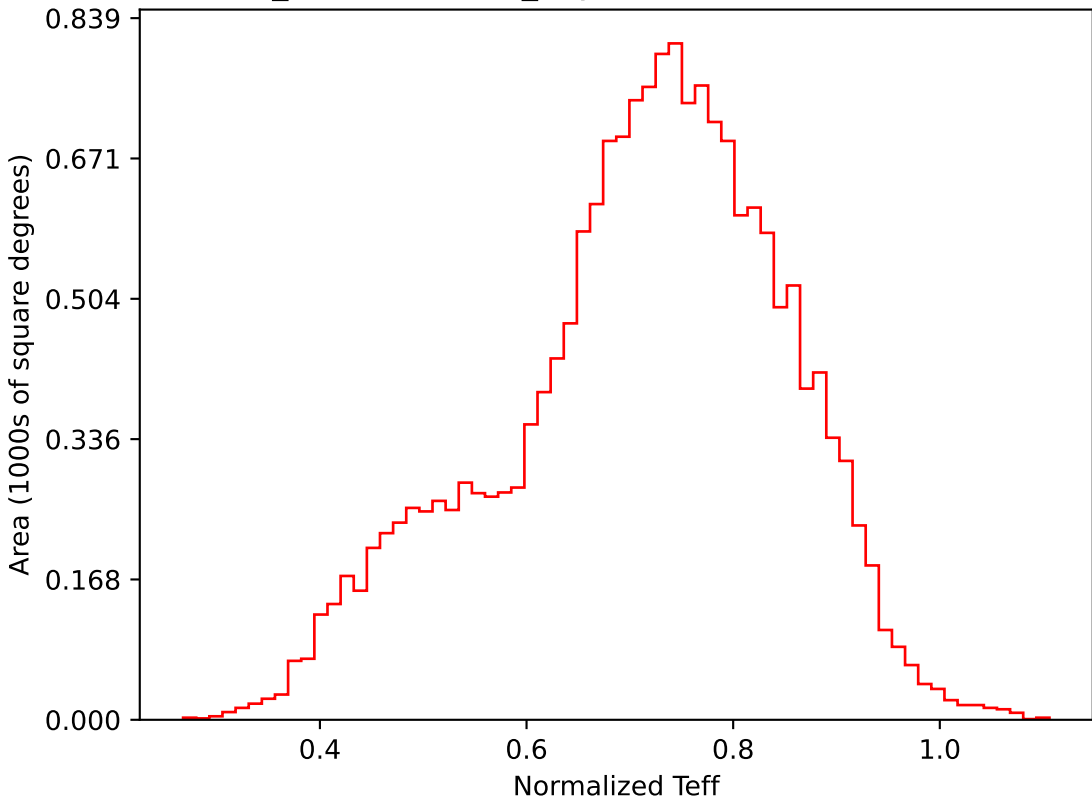
weather_cloudso35v3.4_10yrs WFD i band: Normalized Teff
