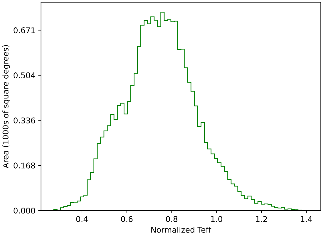
weather_cloudso35v3.4_10yrs WFD g band: Normalized Teff
