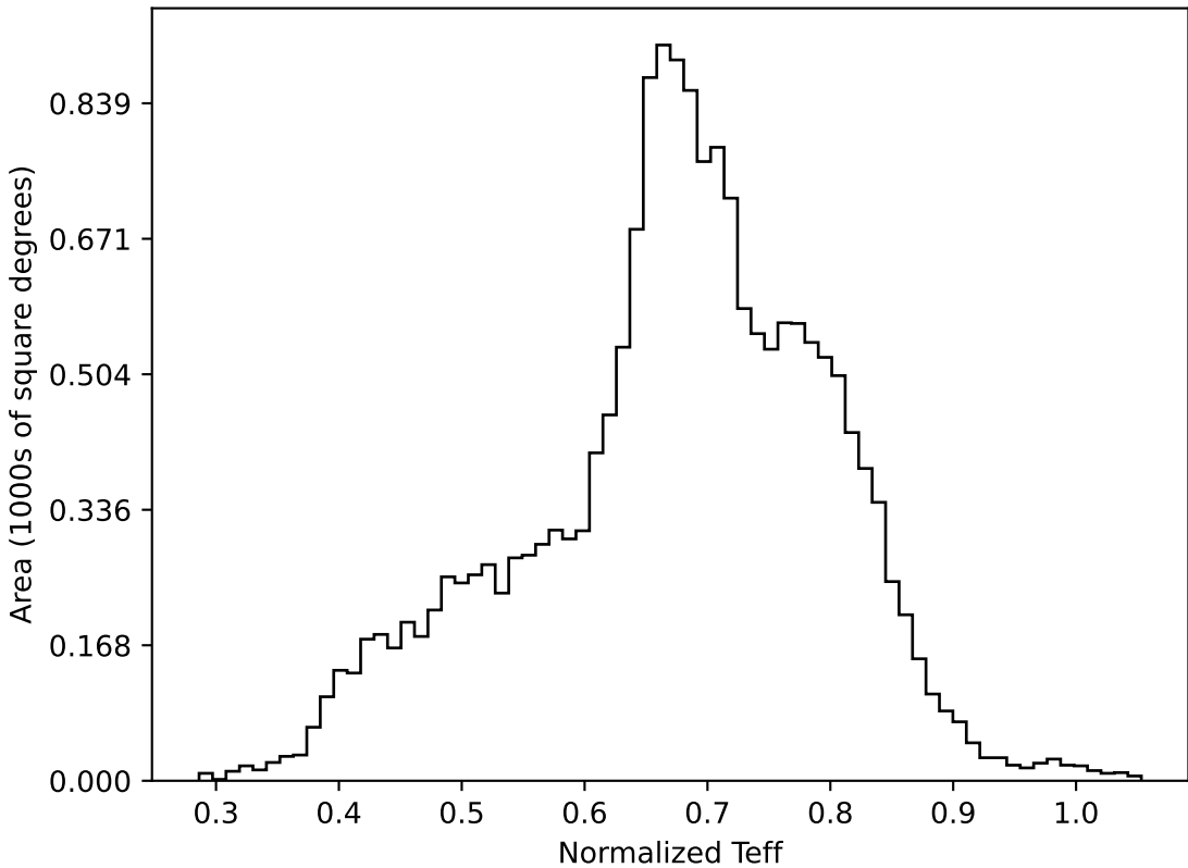
weather_cloudso35v3.4_10yrs WFD all bands: Normalized Teff
