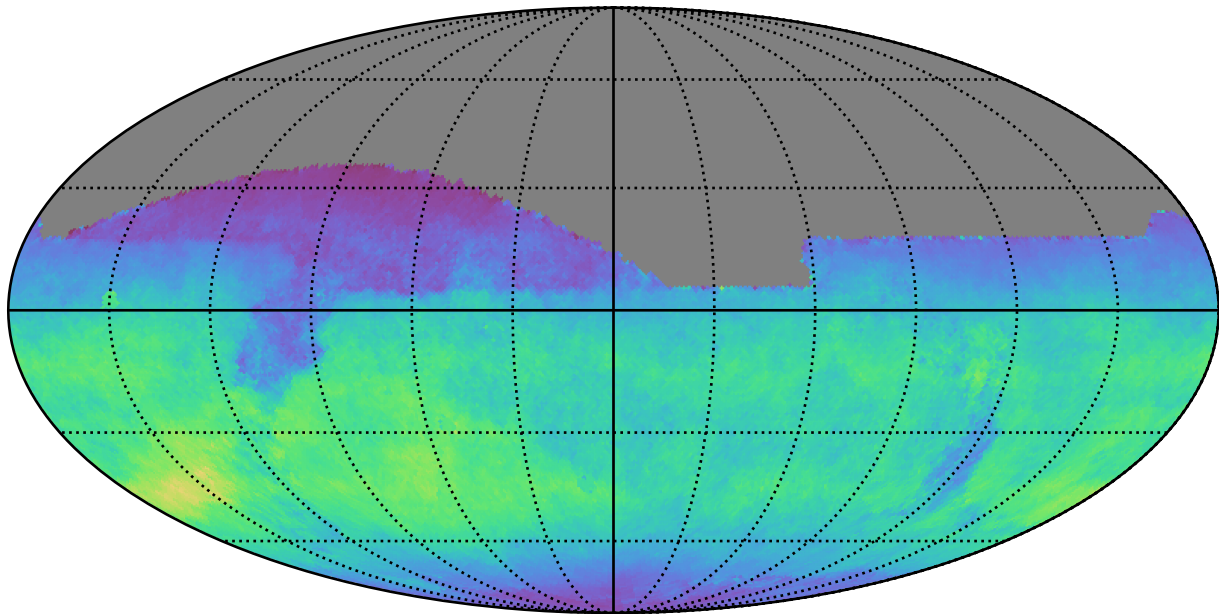
weather_cloudso35v3.4_10yrs All sky z band: Normalized Teff
