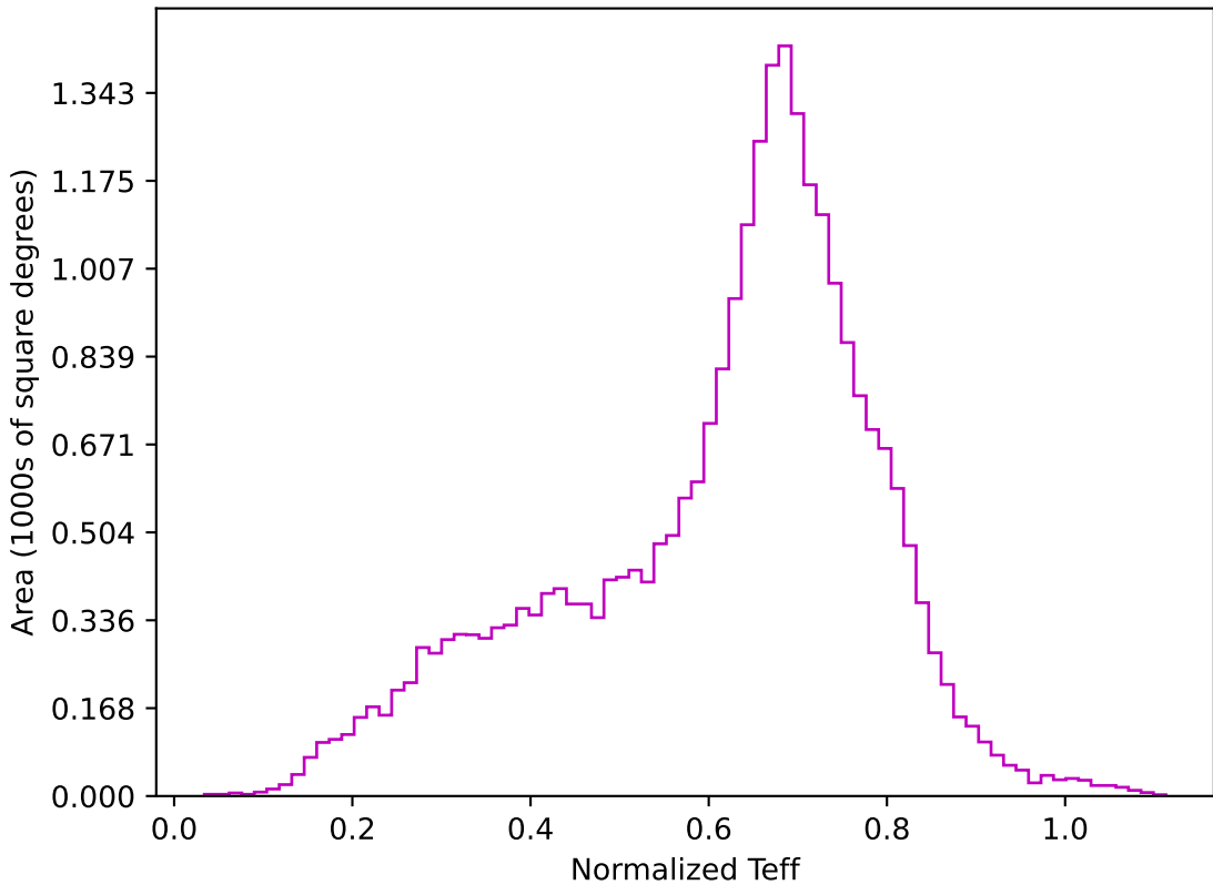
weather_cloudso35v3.4_10yrs All sky z band: Normalized Teff
