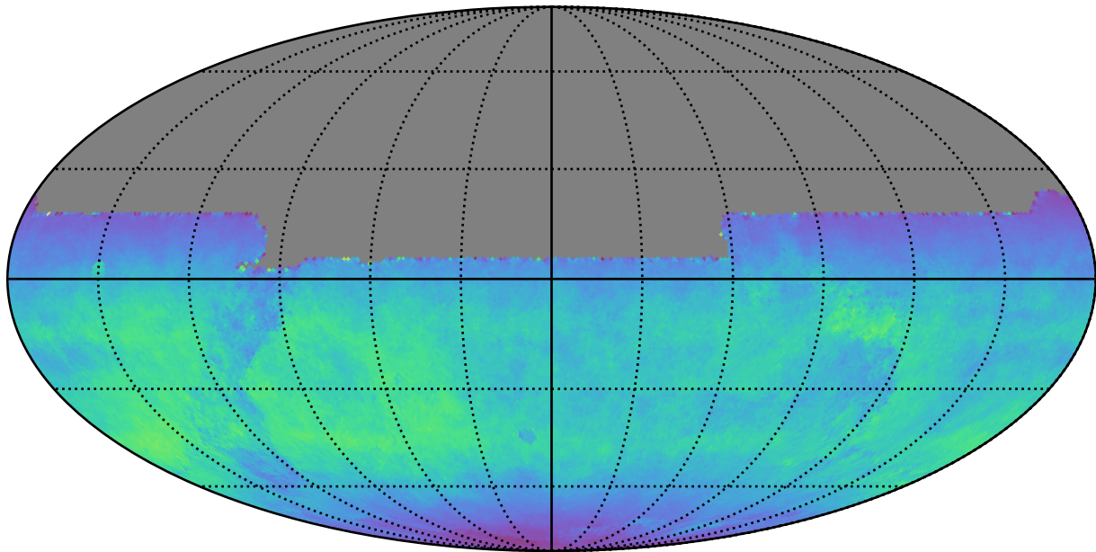
weather_cloudso35v3.4_10yrs All sky y band: Normalized Teff
