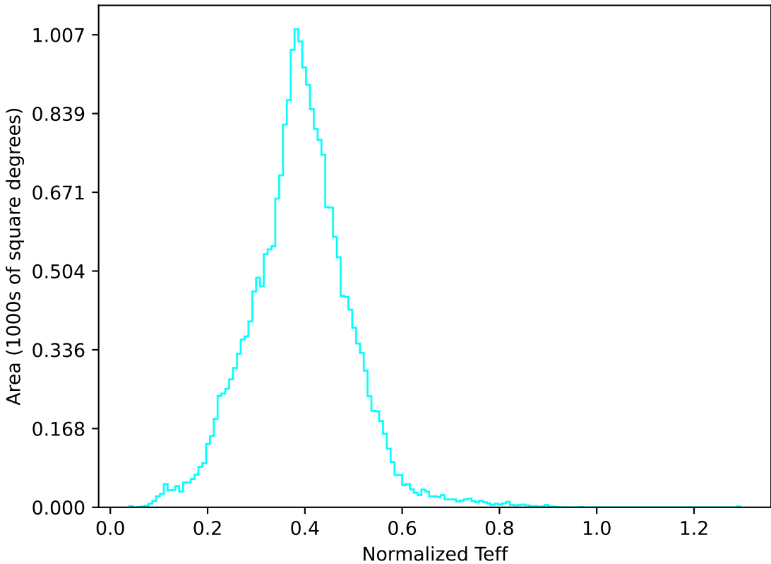
weather_cloudso35v3.4_10yrs All sky u band: Normalized Teff
