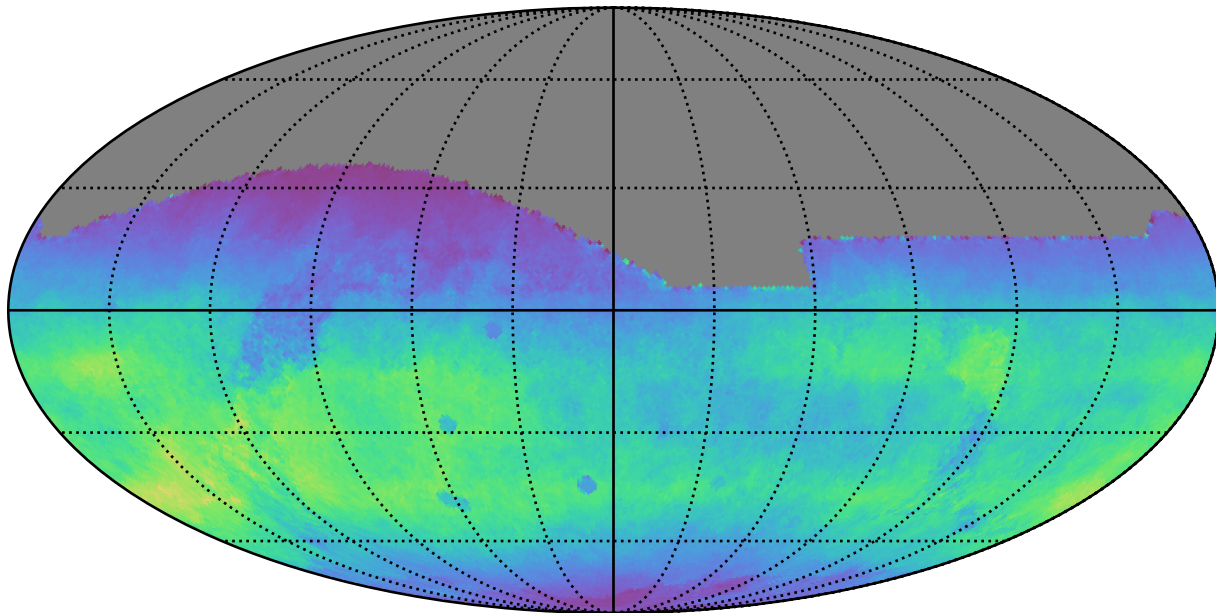
weather_cloudso35v3.4_10yrs All sky r band: Normalized Teff
