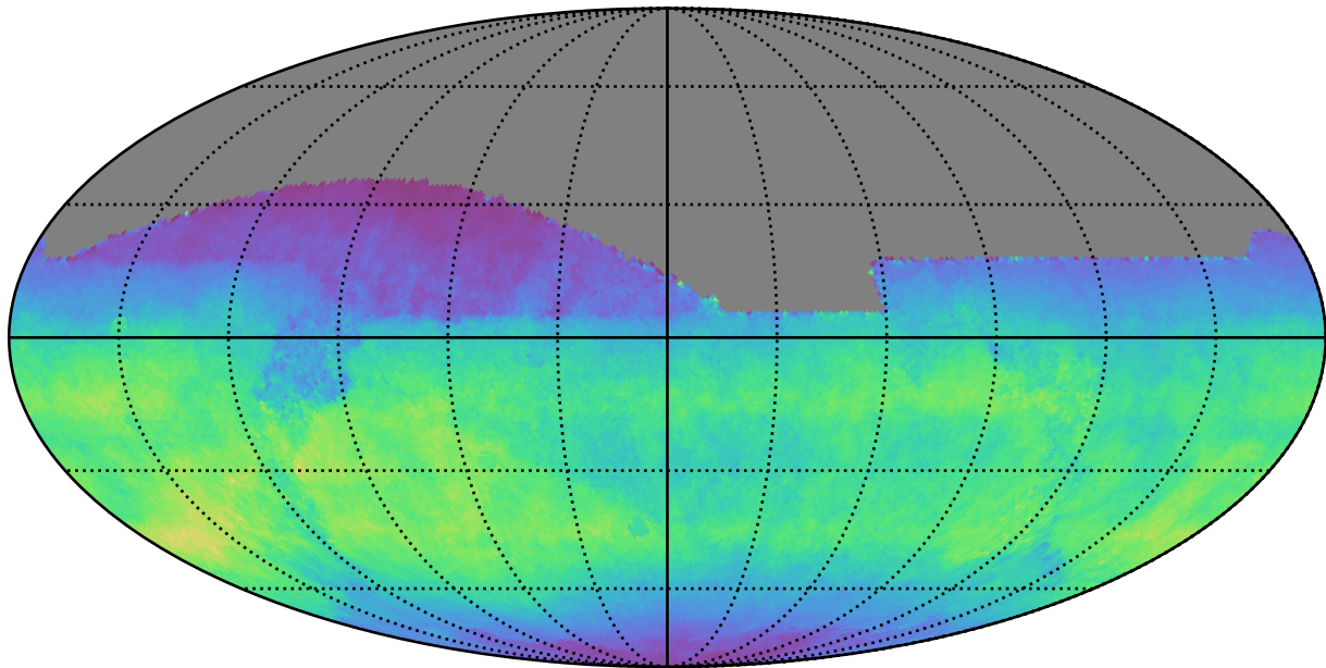
weather_cloudso35v3.4_10yrs All sky i band: Normalized Teff
