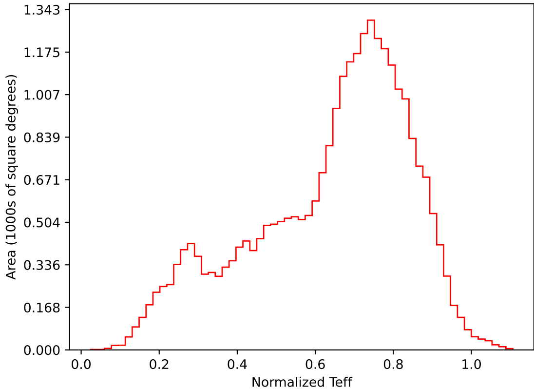
weather_cloudso35v3.4_10yrs All sky i band: Normalized Teff
