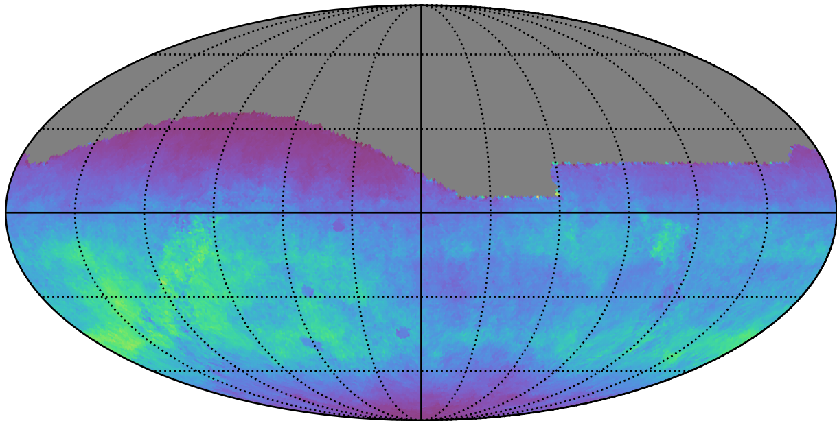
weather_cloudso35v3.4_10yrs All sky g band: Normalized Teff
