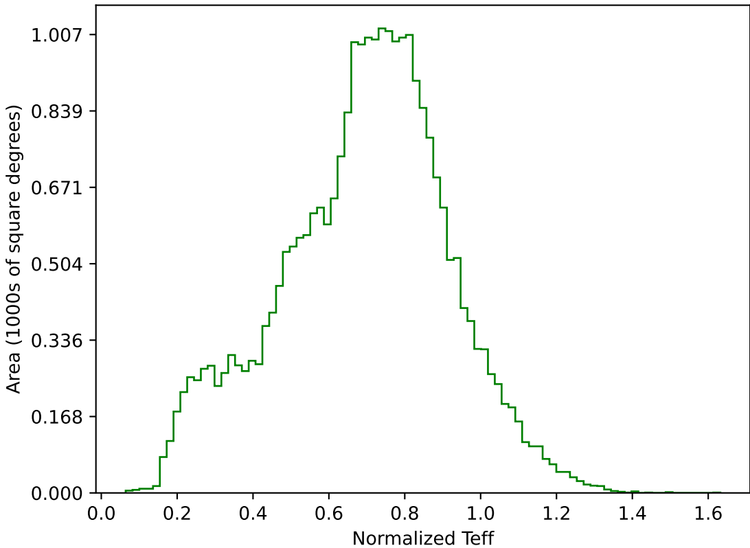
weather_cloudso35v3.4_10yrs All sky g band: Normalized Teff
