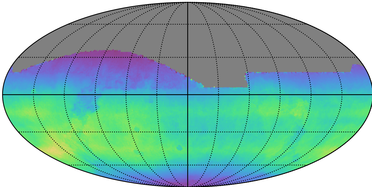
weather_cloudso35v3.4_10yrs All sky all bands: Normalized Teff
