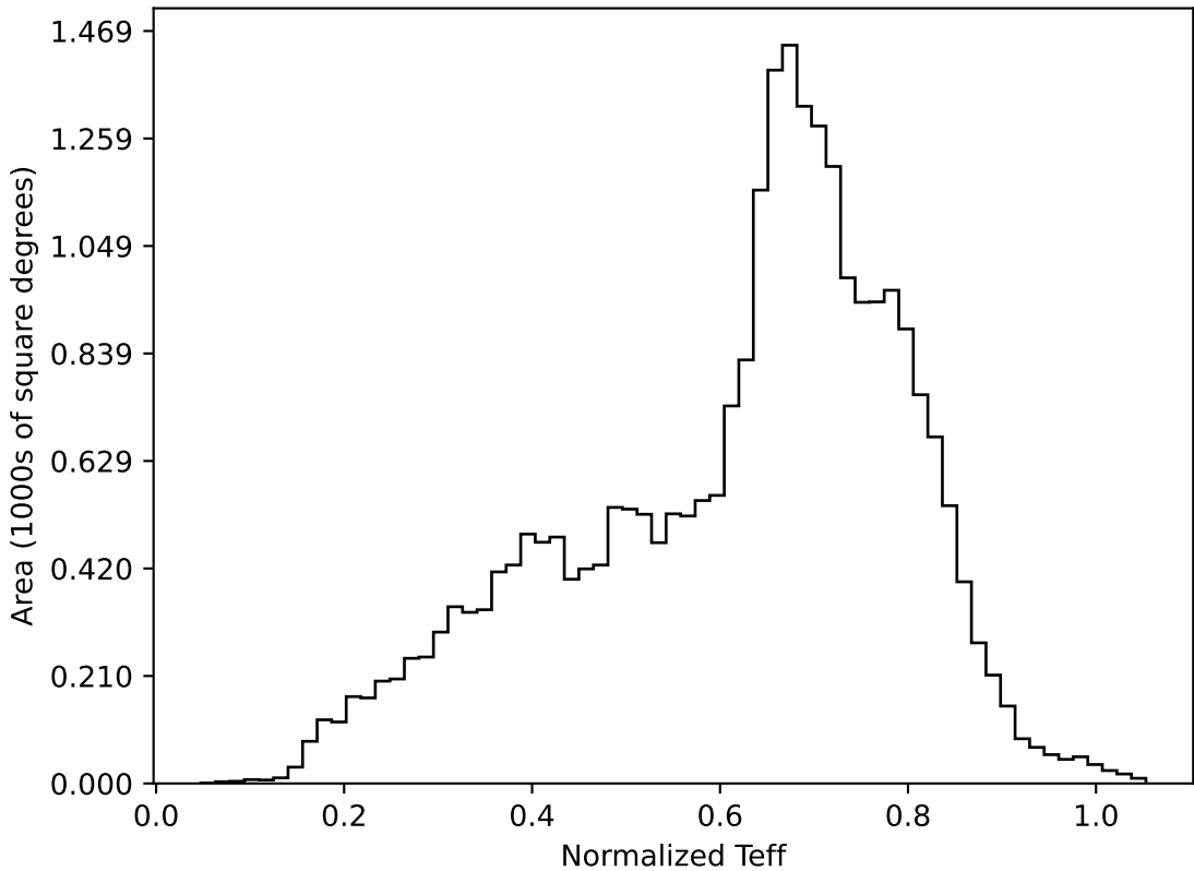
weather_cloudso35v3.4_10yrs All sky all bands: Normalized Teff
