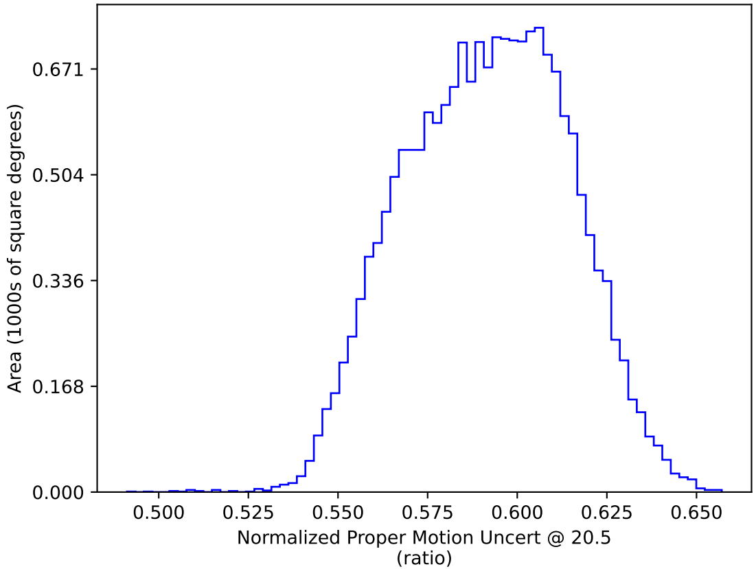
weather_cloudso35v3.4_10yrs WFD: Normalized Proper Motion Uncert @ 20.5
