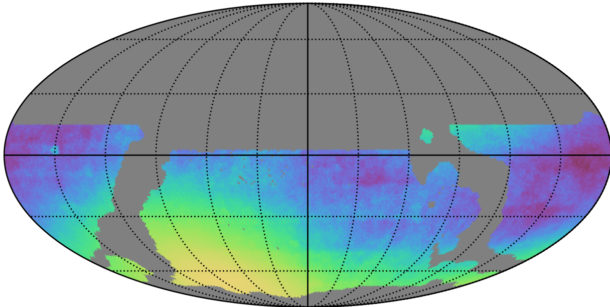
weather_cloudso35v3.4_10yrs WFD: Normalized Parallax Uncert @ 24.0
