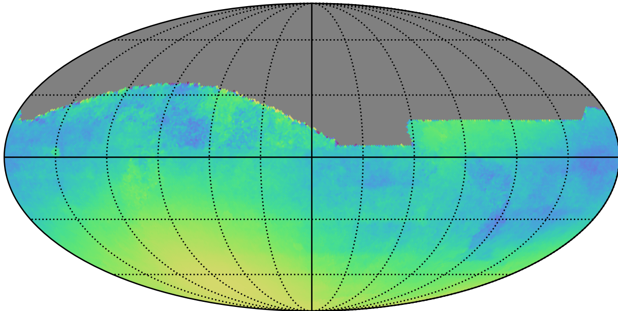
weather_cloudso35v3.4_10yrs All sky: Normalized Parallax Uncert @ 24.0
