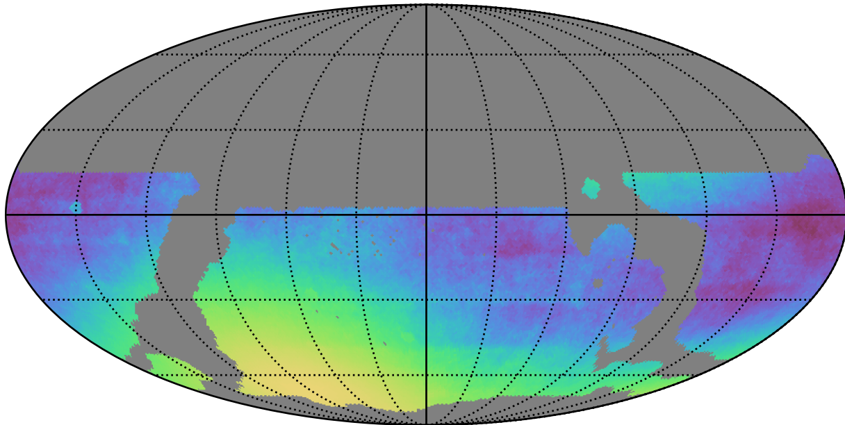
weather_cloudso35v3.4_10yrs WFD: Normalized Parallax Uncert @ 22.4
