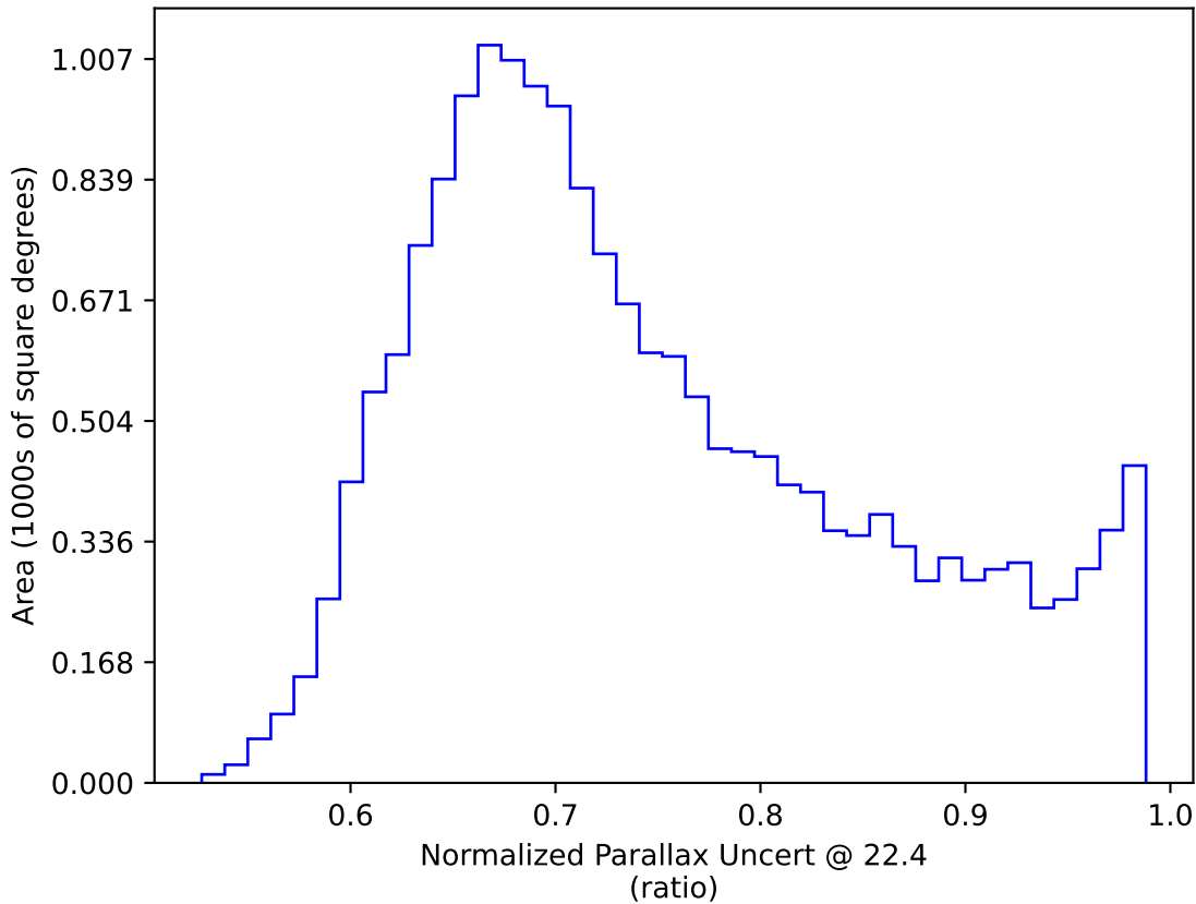
weather_cloudso35v3.4_10yrs WFD: Normalized Parallax Uncert @ 22.4
