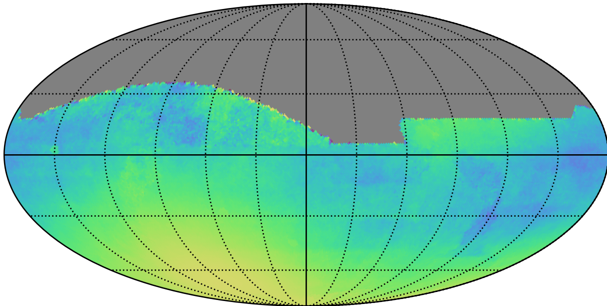
weather_cloudso35v3.4_10yrs All sky: Normalized Parallax Uncert @ 22.4
