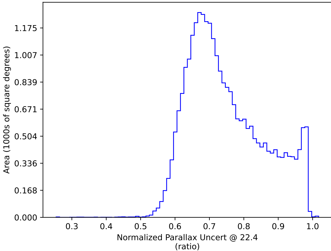
weather_cloudso35v3.4_10yrs All sky: Normalized Parallax Uncert @ 22.4
