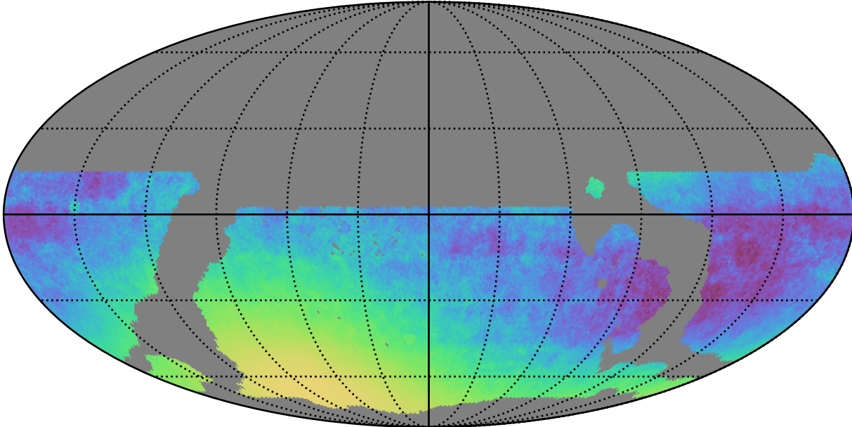
weather_cloudso35v3.4_10yrs WFD y band only: Normalized Parallax Uncert @ 21.3
