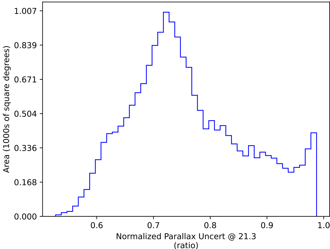
weather_cloudso35v3.4_10yrs WFD y band only: Normalized Parallax Uncert @ 21.3
